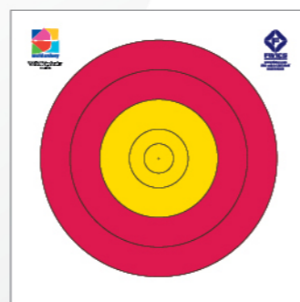
PT 013F TRAINING 122cm-CenterSpot Target Face(7Line) Range : 90m/70m/60m Mark dimension : 48.8cmX48.8cm Total dimension : 61cmX61cm(width/length)
