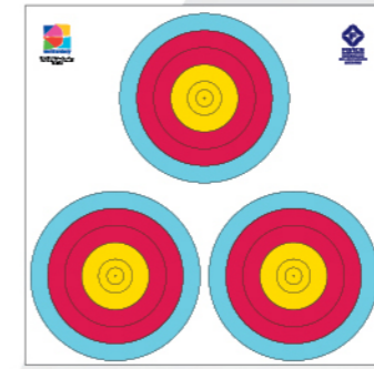
PT 006F OUTDOOR Triangular Target face(5Line) Range : 30m / 20m Mark dimension : (40cm-Center X 3Target) Total dimension : 85cm X 85cm (width/length)
